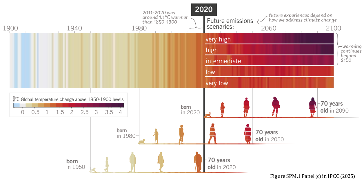
Figure SPM.1 Panel (c) in IPCC (2023)
